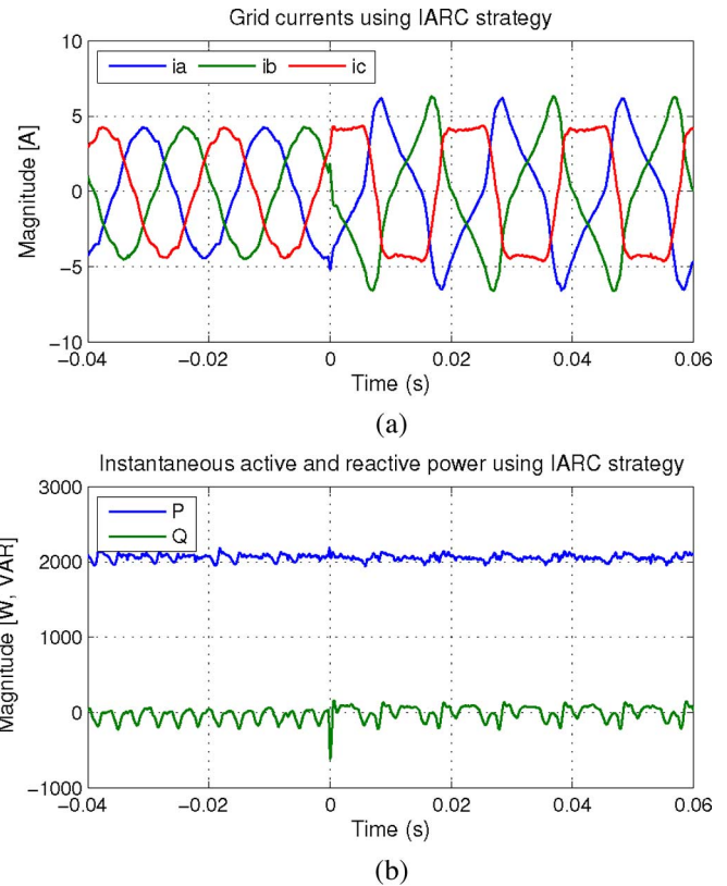
Fig. 11. Experimental results in the case of a single-phase-to-ground fault using IARC: (a) grid currents and (b) active and reactive powers that are delivered to the utility network.
